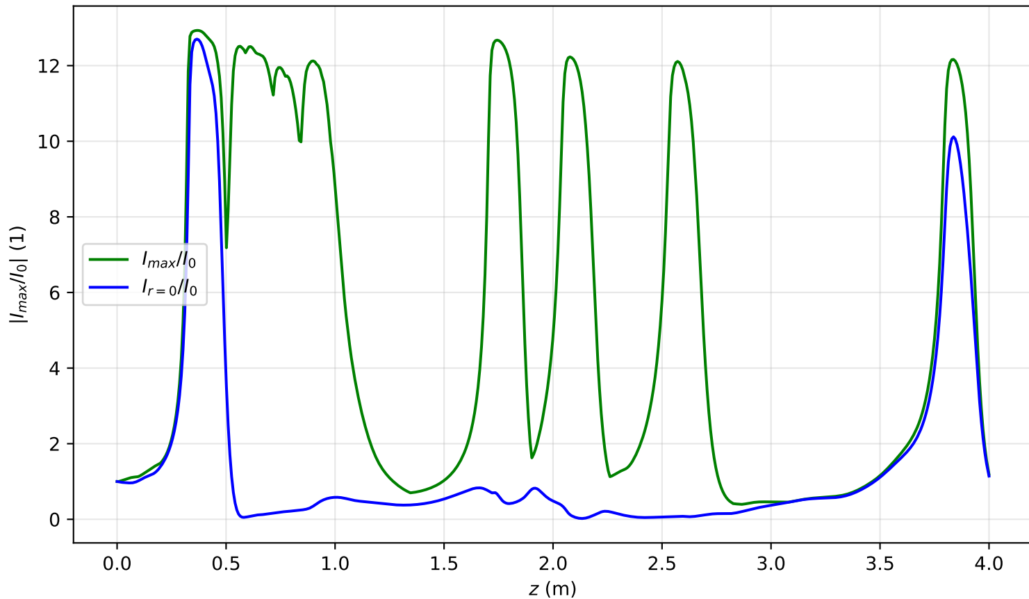
I_{max}(x = 0, y = 0, z)/I_0 , Pin=8.6Pcr, noisy input, artificial time
